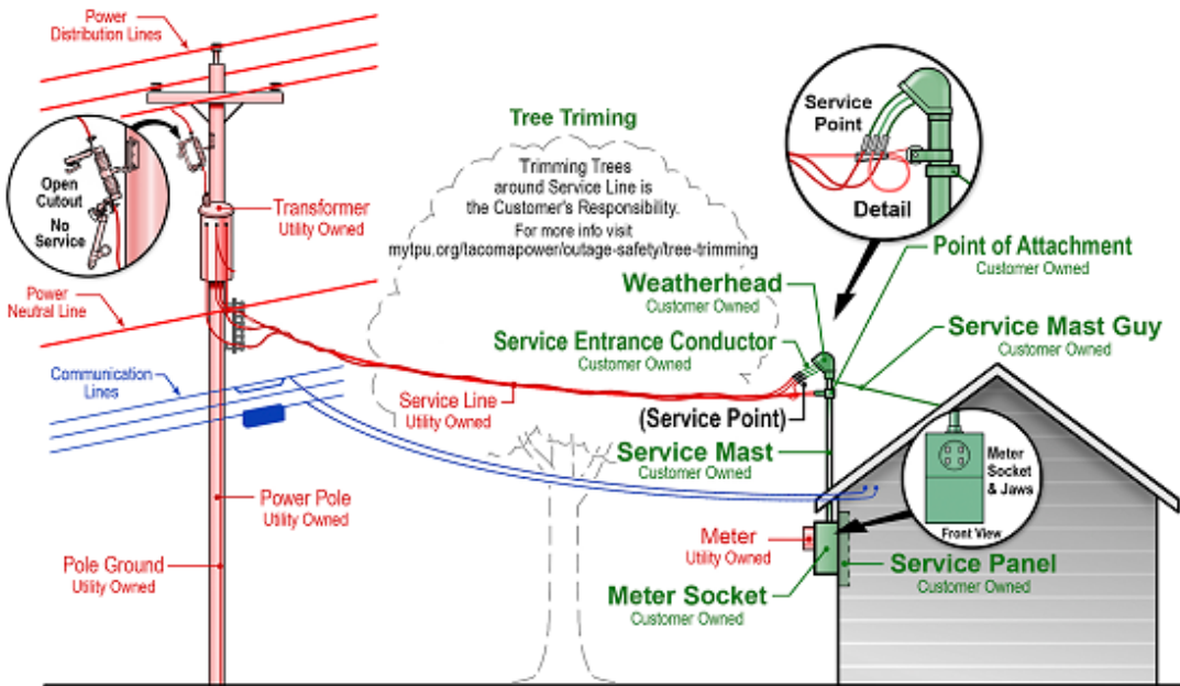
Utility Owned and Customer Owned Equipment
